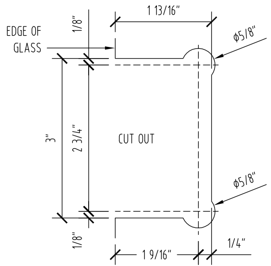
GLASS FABRICATION TEMPLATE
