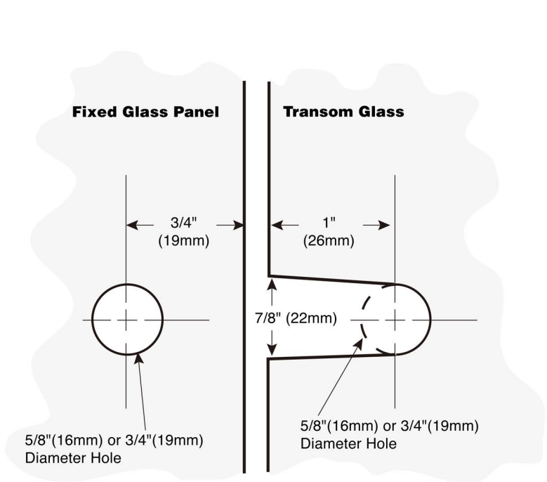
TEMPLATE FOR FIXED GLASS PANEL TO MOVABLE TRANSOM GLASS
