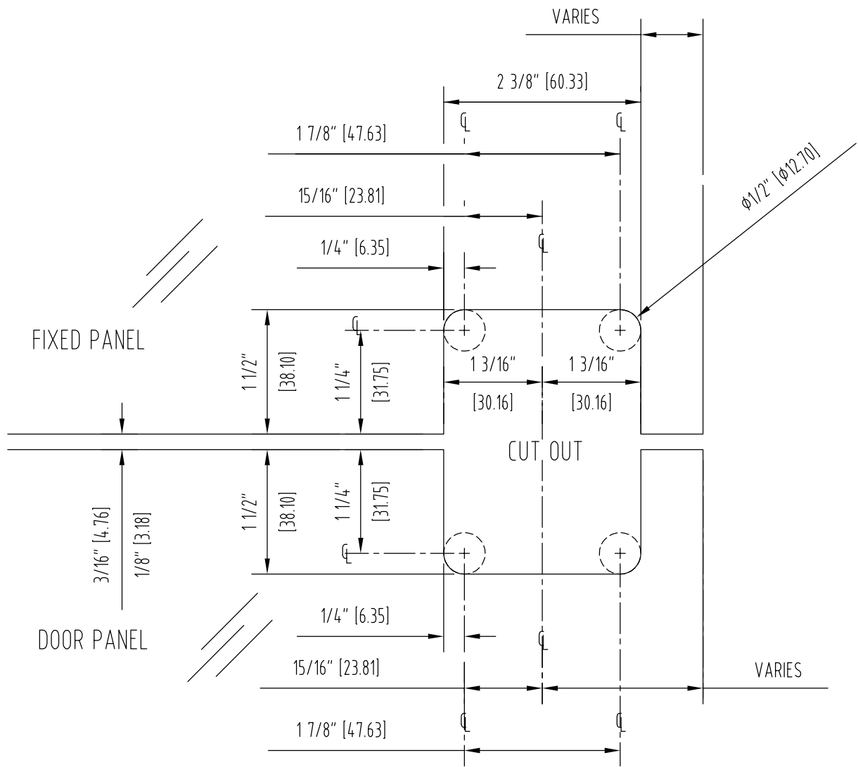
INSET MOUNT METHOD 1/8" (3mm) TO 3/16" (5mm) CLEARANCE GLASS FABRICATION TEMPLATE
