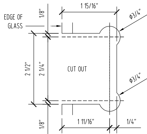
FIXED PANEL GLASS FABRICATION TEMPLATE
