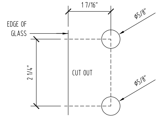
GLASS FABRICATION TEMPLATE FIXED PANEL
