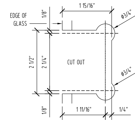
FIXED PANEL GLASS FABRICATION TEMPLATE
