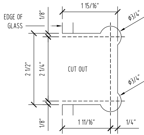
GLASS FABRICATION TEMPLATE 1 OF 2
