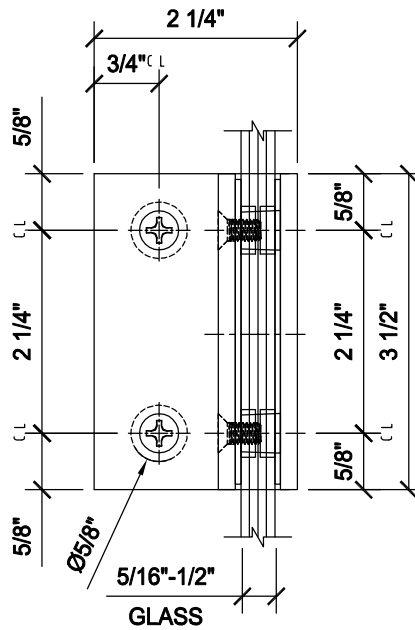
GLASS FABRICATION TEMPLATE 1 OF 2
