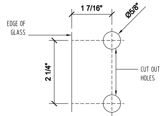
FIXED PANEL GLASS TEMPLATE
