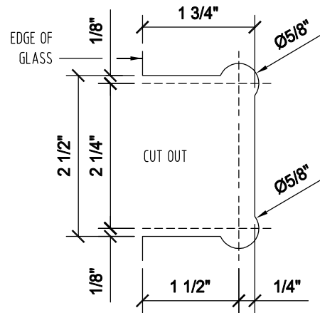
GLASS FABRICATION TEMPLATE 1 OF 2
