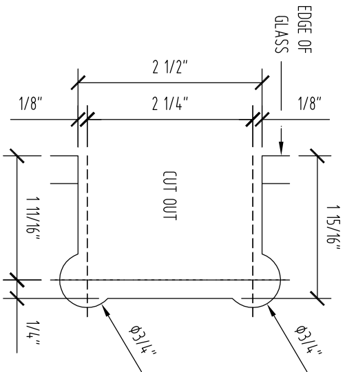
FIXED PANEL GLASS FABRICATION TEMPLATE
