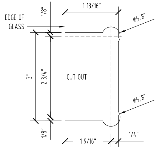
TEMPLATE FOR DOOR AND FIXED PANEL ARE THE SAME
