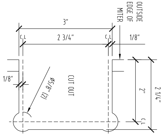
FIXED PANEL TEMPLATE
